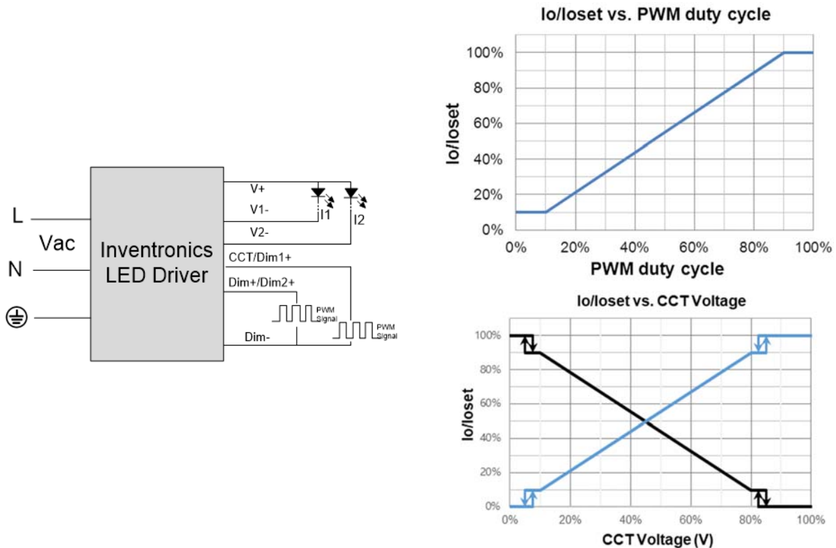
Implementation 5: Positive logic
