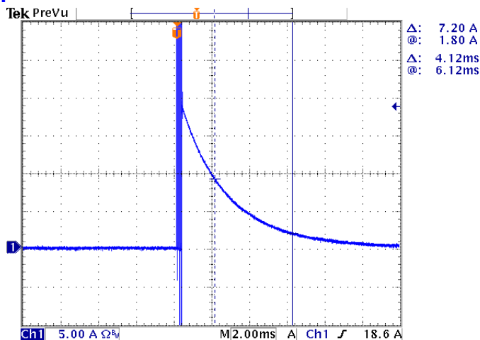
ESM-480S140BG( I_o=1050mA )
